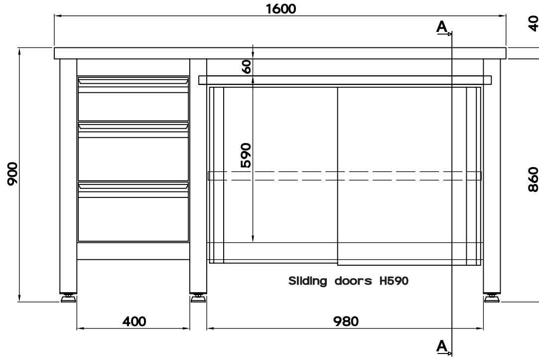
Vista frontale - Front view
